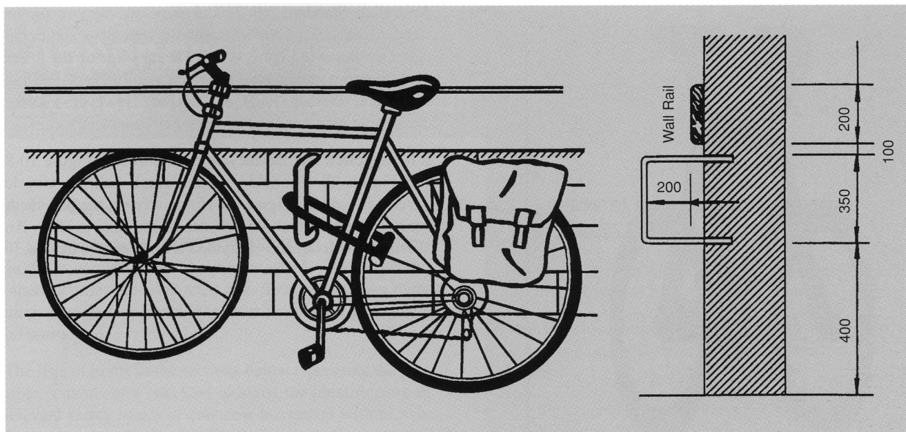
Figure 10-14: Wall Mounted Bracket and Rail
