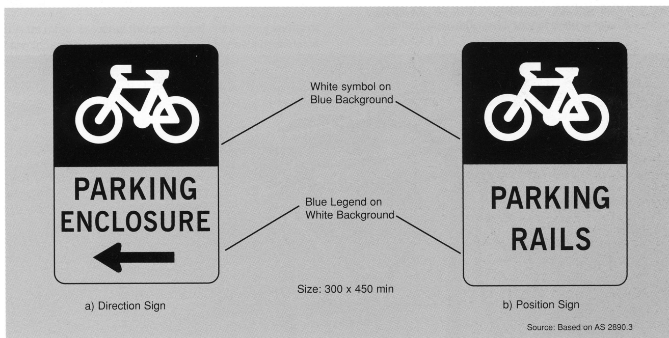
Figure 10-15: Information Signs for Bicycle Parking Facilities
