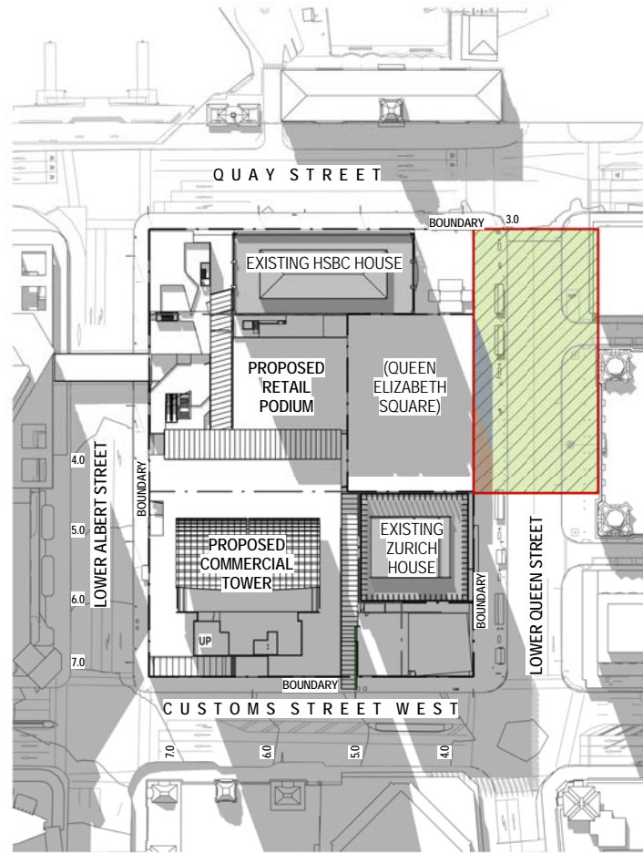
3 Sun Study - April 1 @ 12:30pm A04-S51 1:1000
