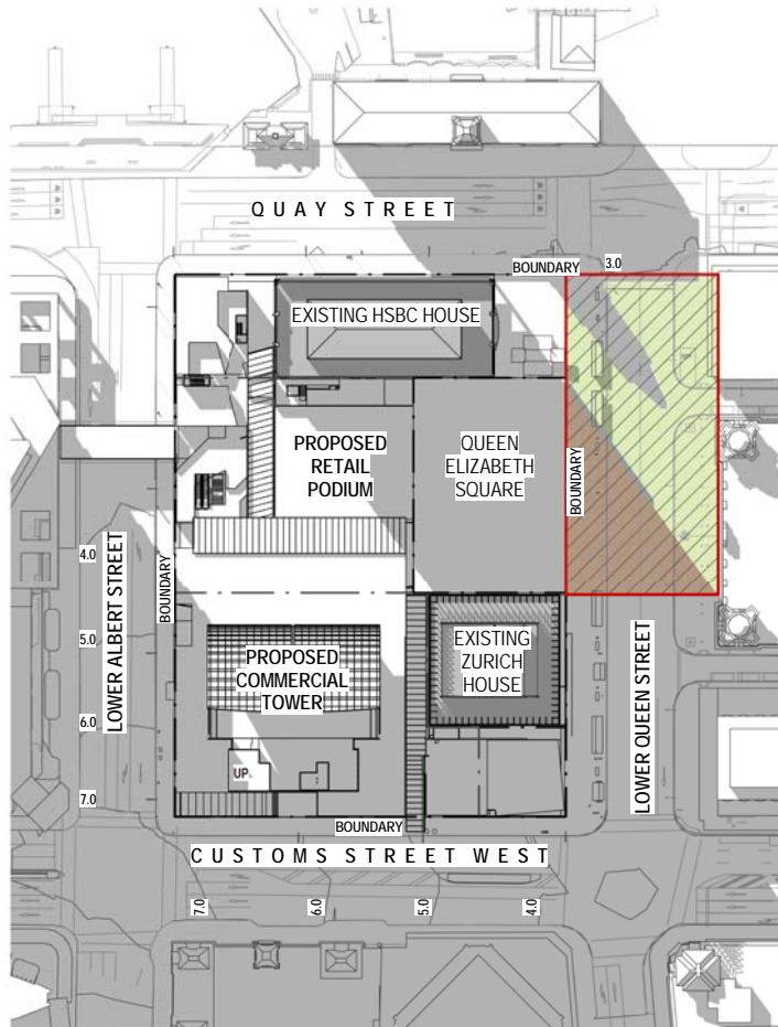
5 Sun Study - June 21 @ 1:30pm A04-S51 1:1000
