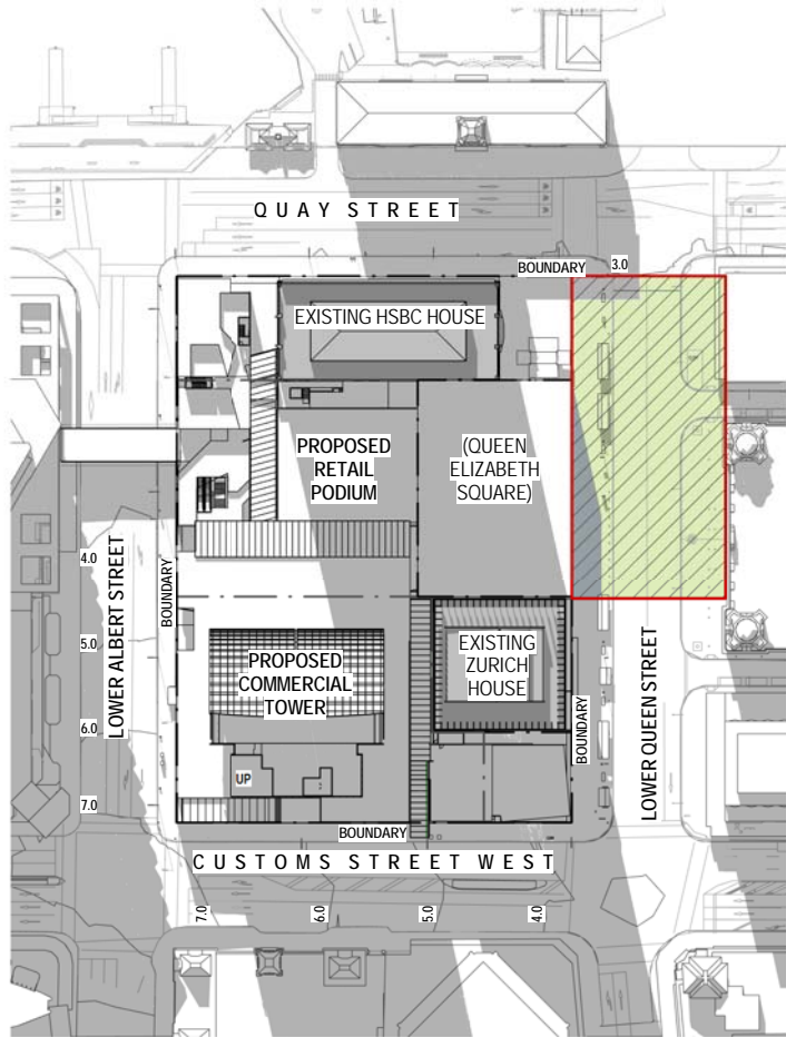
2 Sun Study - June 21 @ 12:00pm A04-S51 1:1000
