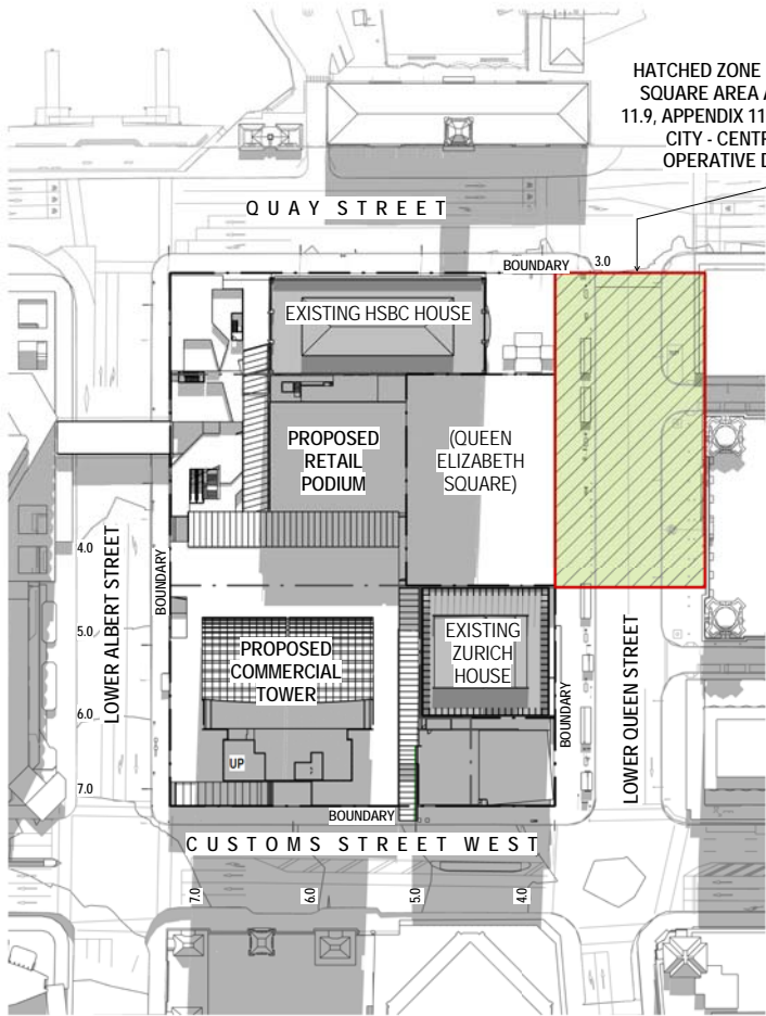
1 Sun Study - April 1 @ 11:30am A04-S51 1:1000
