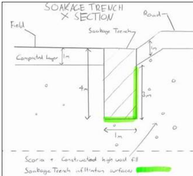
Figure 1: Soakage Trench
