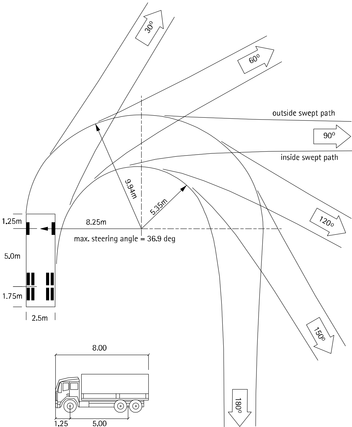
Figure 13.5 90 percentile truck tracking curves
