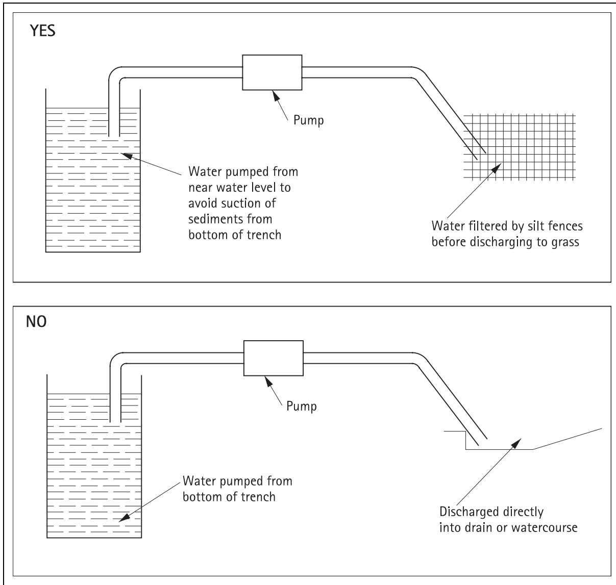
Figure A16.10 Pumping water from the site
