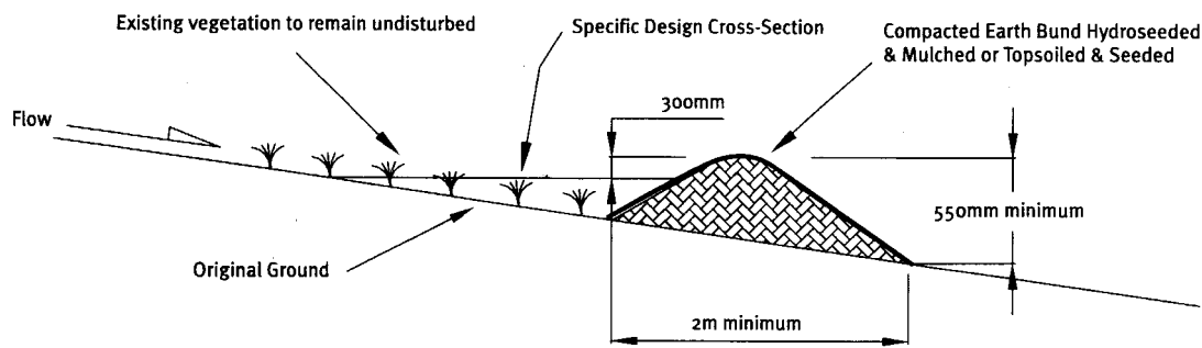
Cross Section of Diversion Bund/Channel
