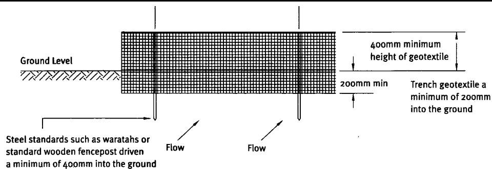
Elevation of Silt Fence
