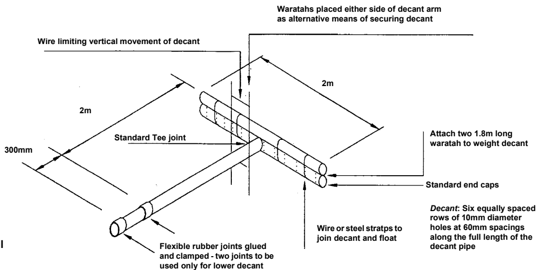
Decant Detail
