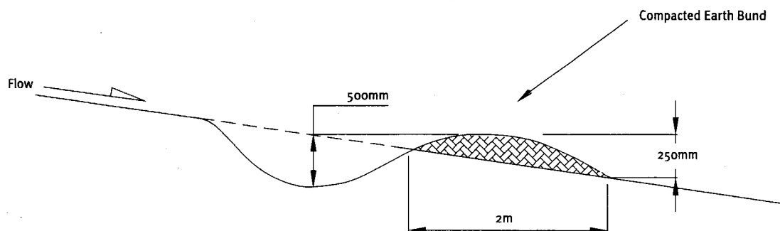
Cross Section of Contour Drain
