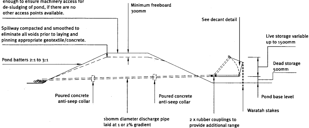
Cross Section of Sediment Pond
