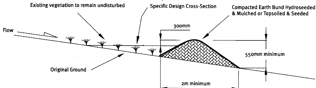
Cross Section of Diversion Bund/Channel
